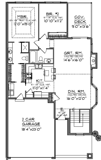
MAIN FLOOR PLAN 1333 SQ. FT.
