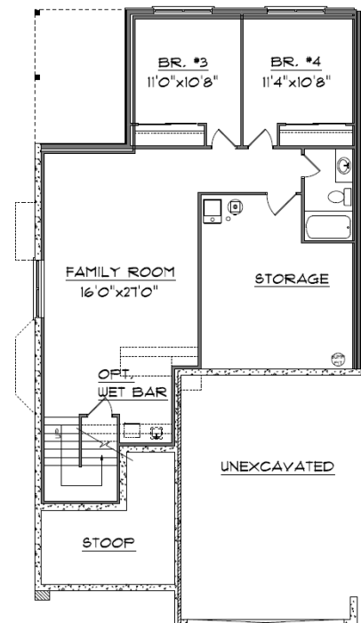
LOWER LEVEL FUTURE FIN: 912 to 920 SQ. FT.
